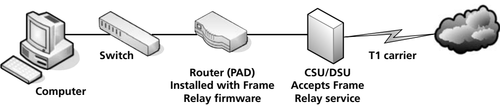
Figure 7-9 Typical T1 configuration with Frame Relay
